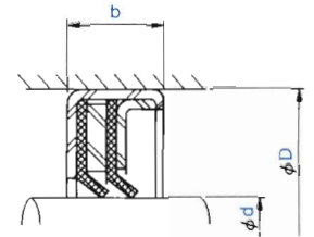
KA3J type
